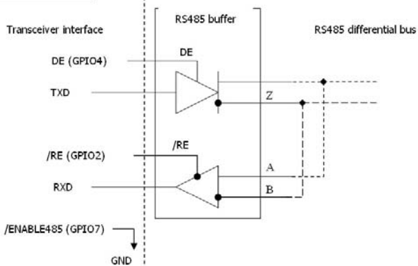
RS485 control lines managed with two different control lines
