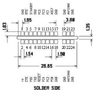
Figure 1: Plugged module mechanical feature
